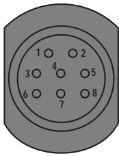
8-Pin Integral or Hanging Connector (male profile) Connection Type 'C', 'H', or 'J' Mating Accessories: • P/N 251135 Field Installable Connector • Extension Cables
